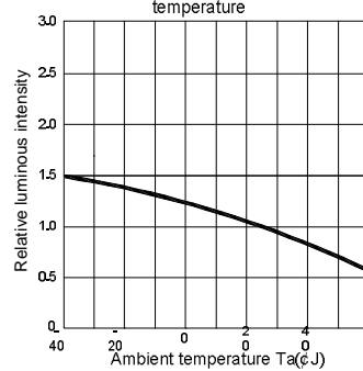
Fig.4 Relative luminous intensity vs. Ambient temperature
