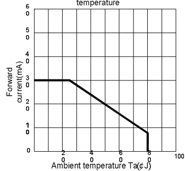
Fig.2 Forward current operating curve vs. Ambient temperature
